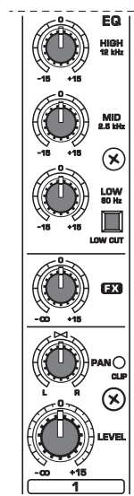
Fig. 2.1: Connectors and controls on the mono channels
